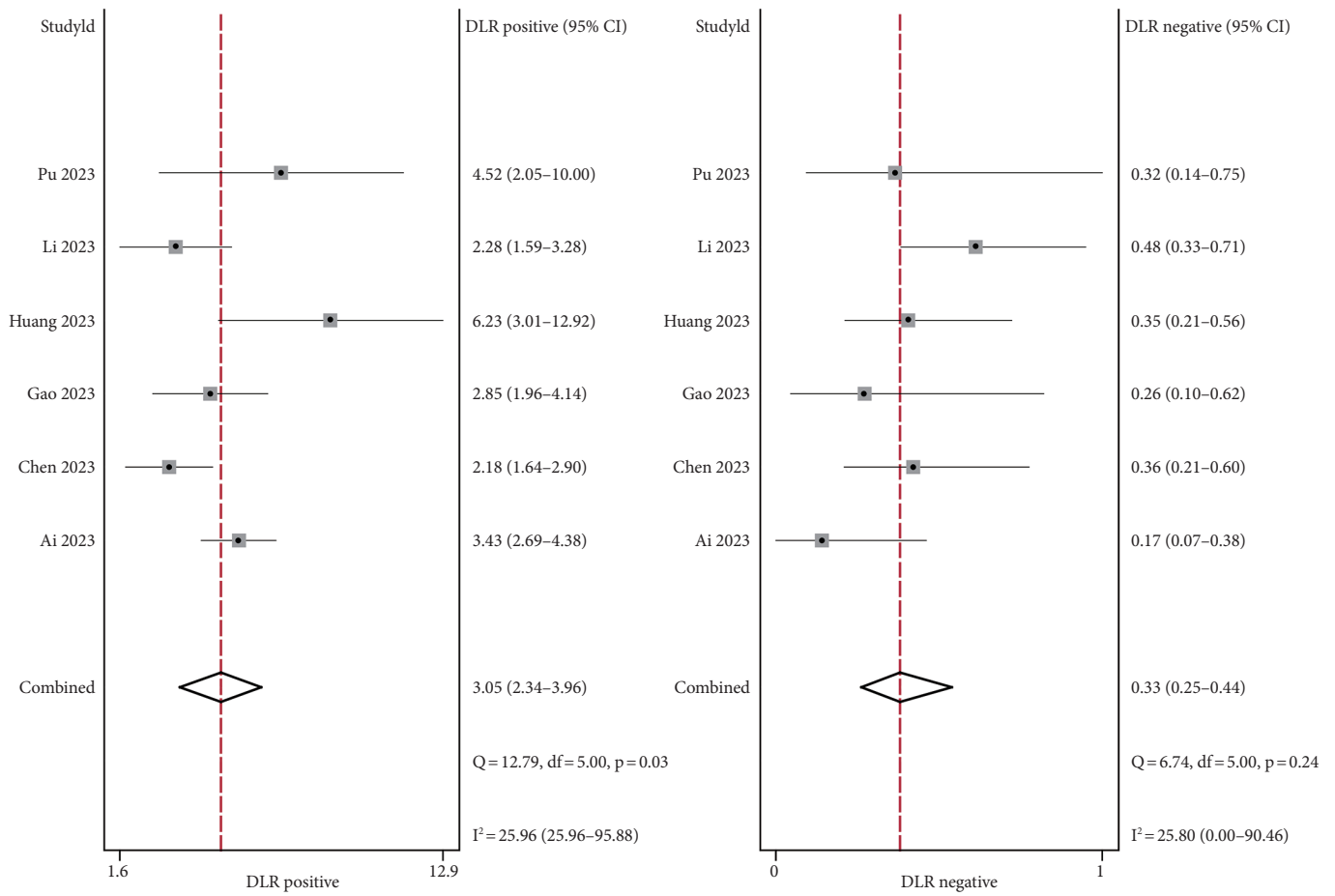
Supplementary Fig. 3. Forest plot of estimates of diagnostic positive likelihood ratio and diagnostic negative likelihood ratio of high vertebral bone quality score for cage subsidence and screw loosening after lumbar surgery. DLR, positive likelihood ratio; CI, confidence interval.
